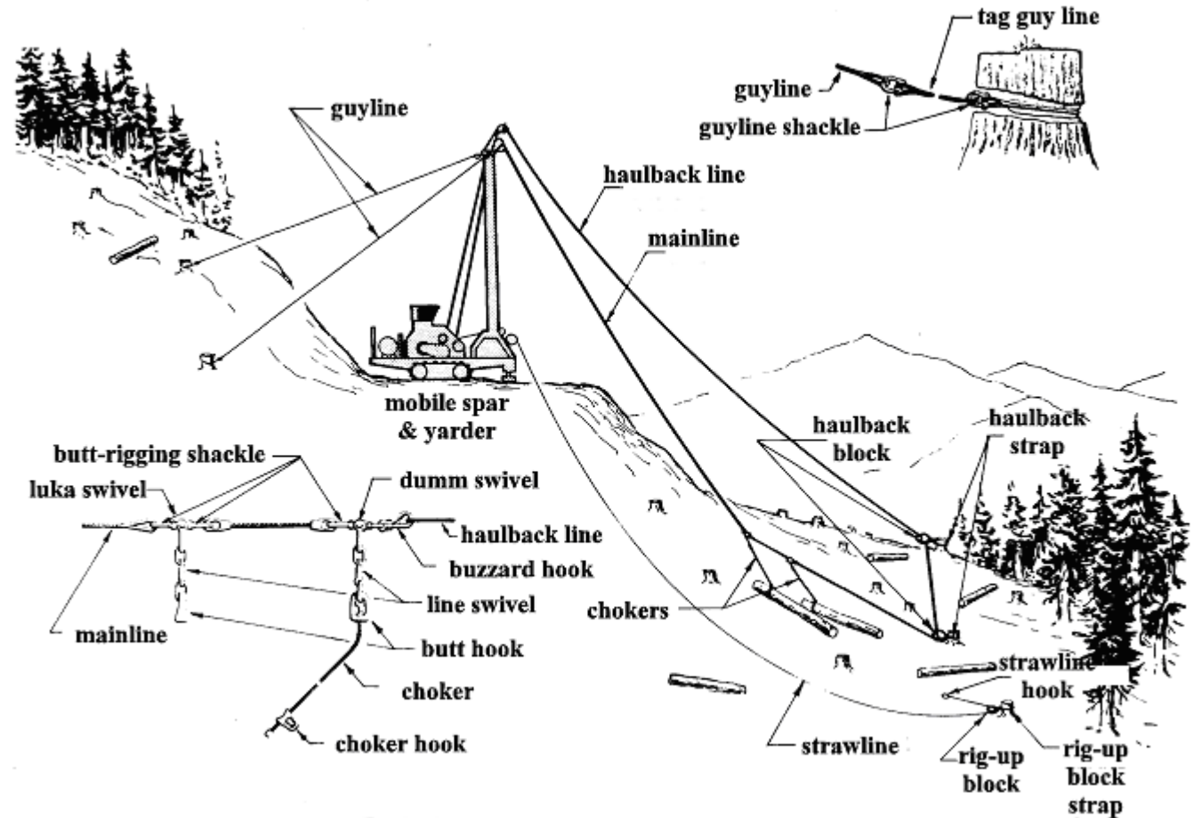
Highlead System (modified after SIMMONS, 1979)
